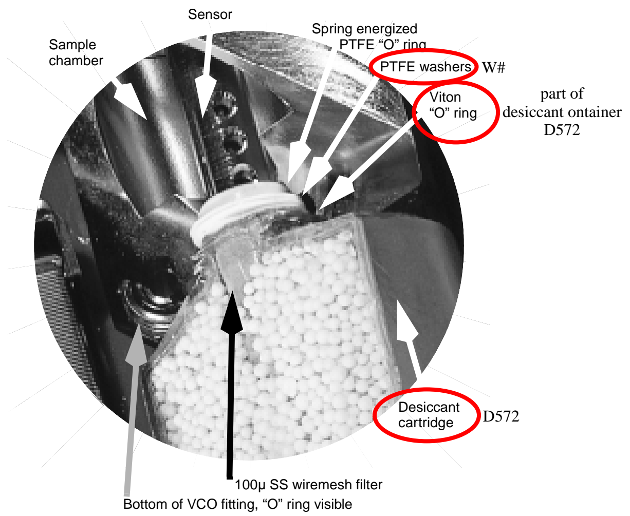
Bottom view of 8800P with cover open. The sample chamber and desiccant cartridge are shown cut open to facilitate an understanding of the mechanism and how it is assembled.
