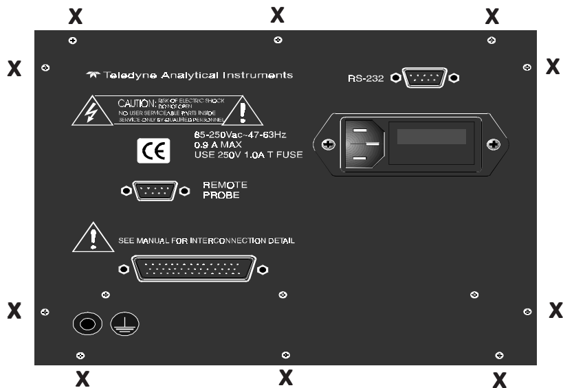
Figure 5-4: Rear-Panel Screws
