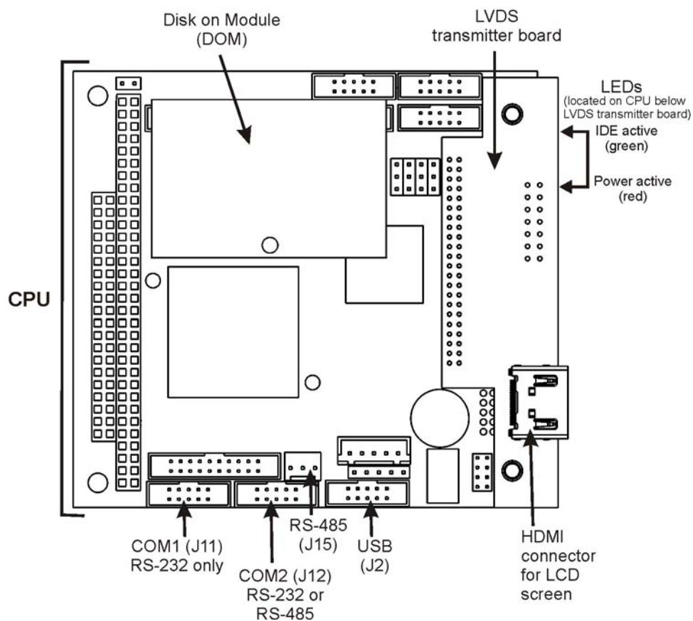
Figure 9-10: CPU Board
