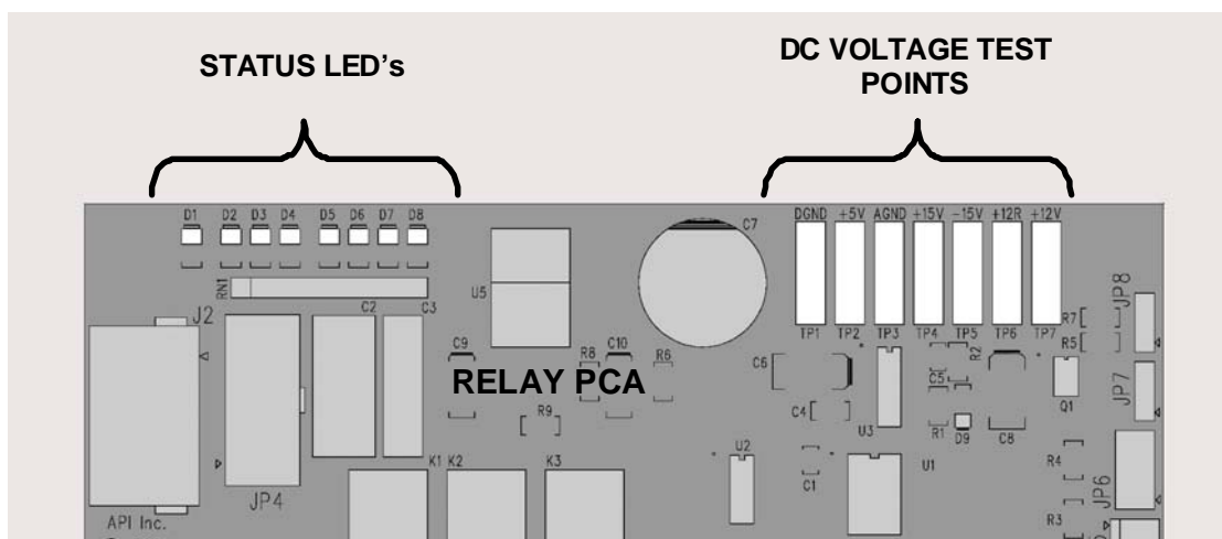
Figure 10-5: Relay Board Status LEDs
