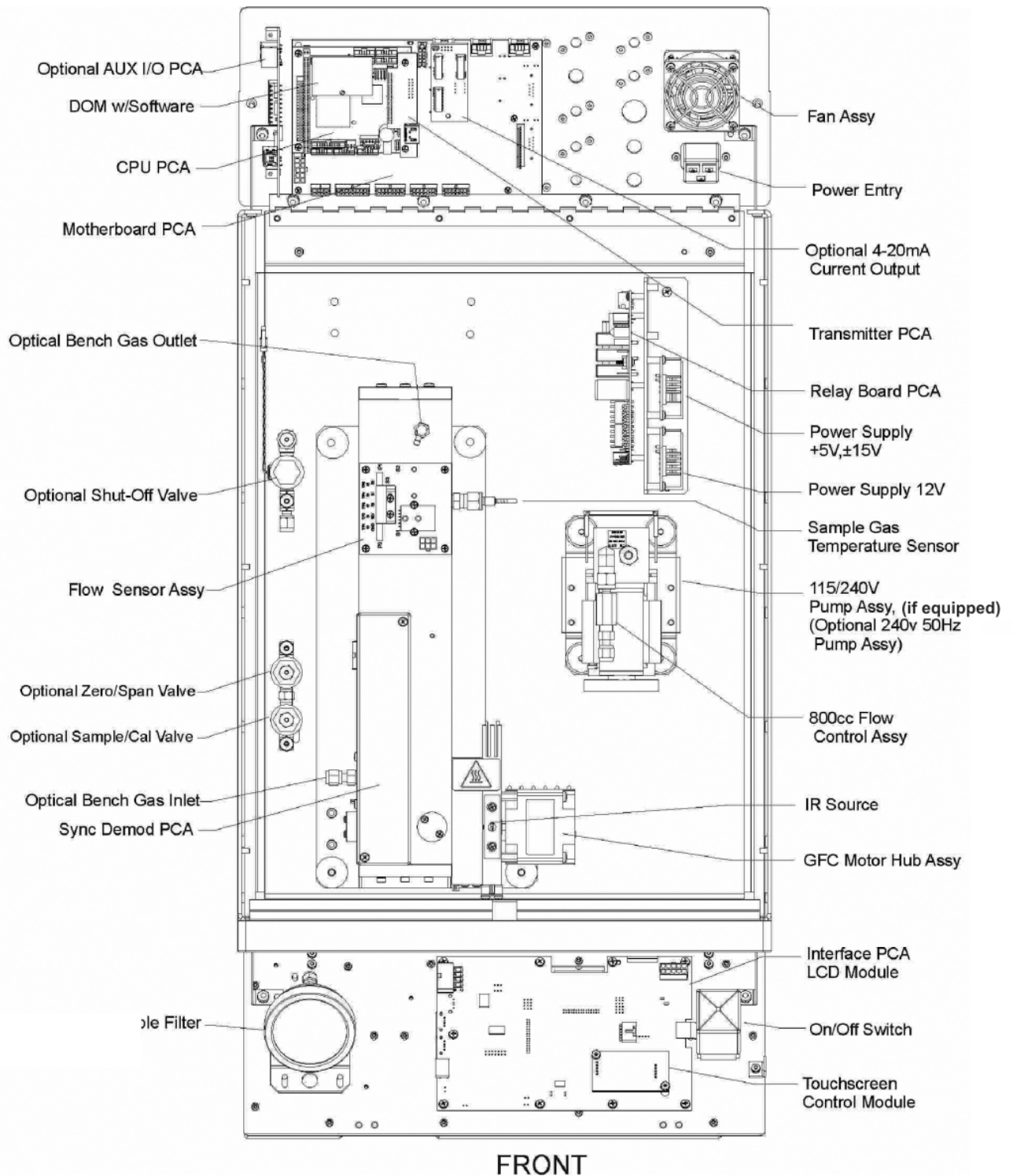
Figure 3-6: Internal Layout – GFC7002TU
