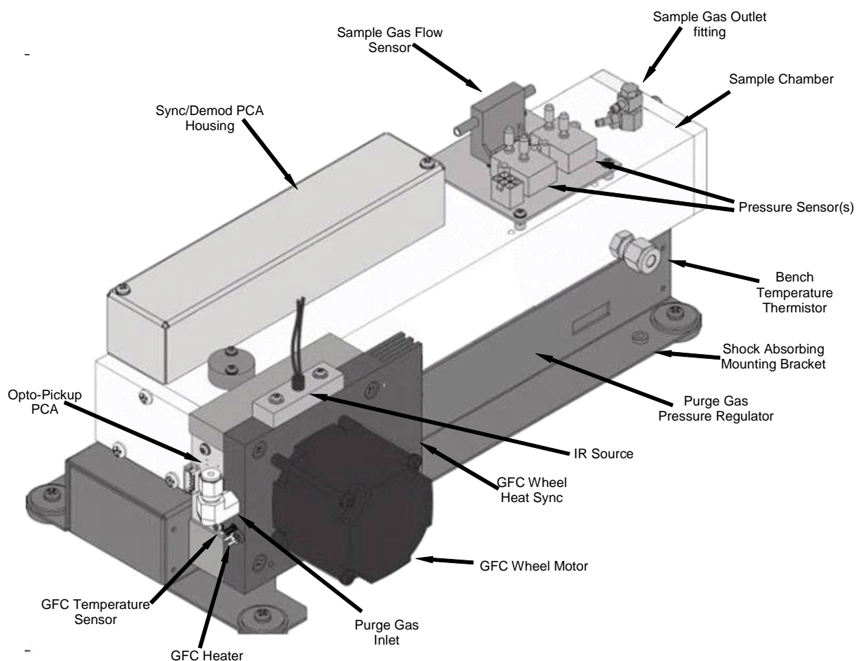
Figure 3-7: Optical Bench Layout (shorter bench, GFC7002TU, shown)
