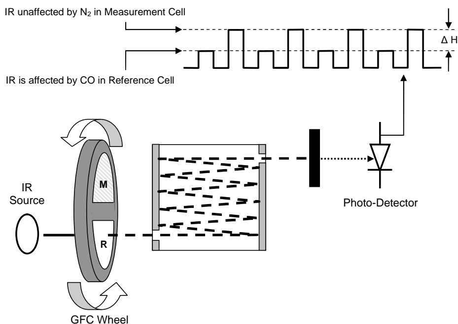
Figure 12-3: Measurement Fundamentals with GFC Wheel
