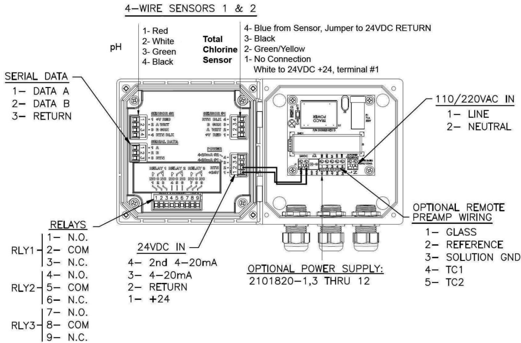
Figure 3-2: TCA330 Wire Transmitter, 24VDC or /110/22 VAC
