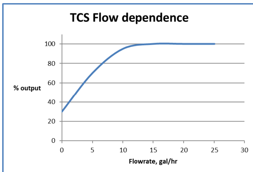
Figure 2.2 TCA330 Flow Dependence
