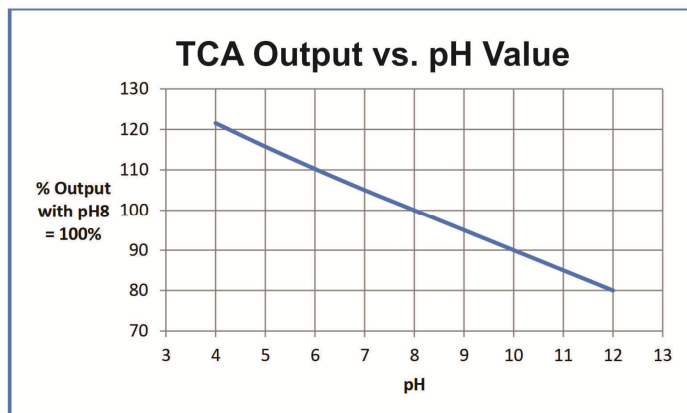
Figure 2-1: TCA Output vs. pH
