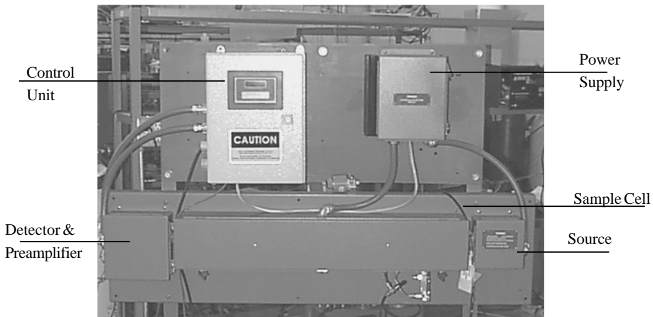
Model 6000B Photometric Analyzer with D2 Lamp Analysis Bench shown with Integral General purpose bulkhead Control Unit
