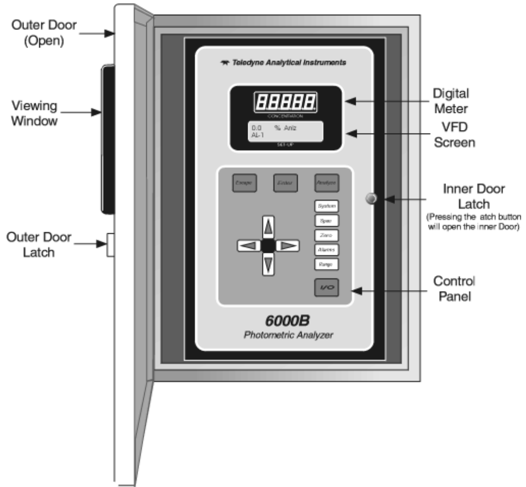
Figure 1-1: Front of Unmounted Control Unit
