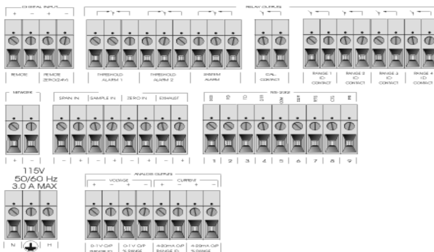
Figure 2-3: Interface Panel of the Model 6000B Control Unit
