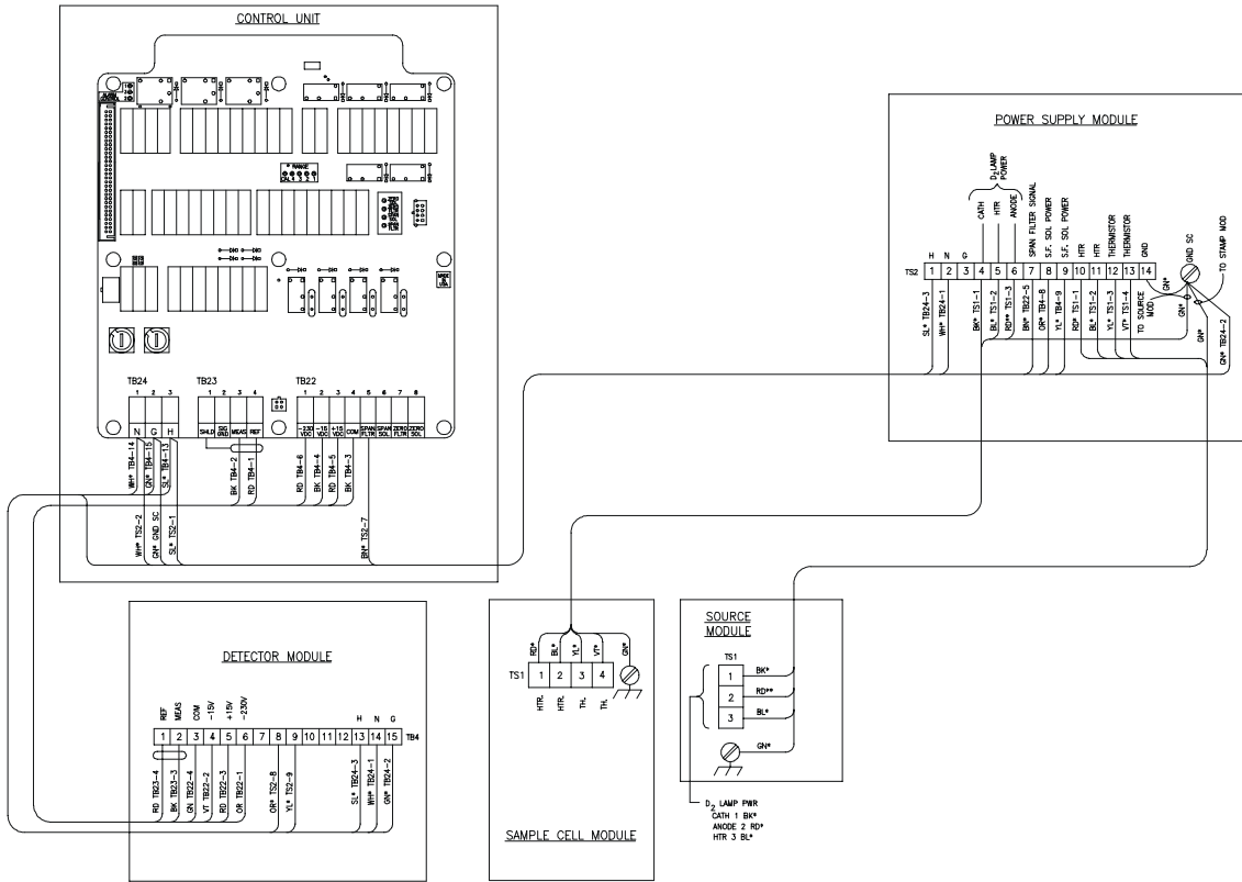
6000B Integral Control Unit
