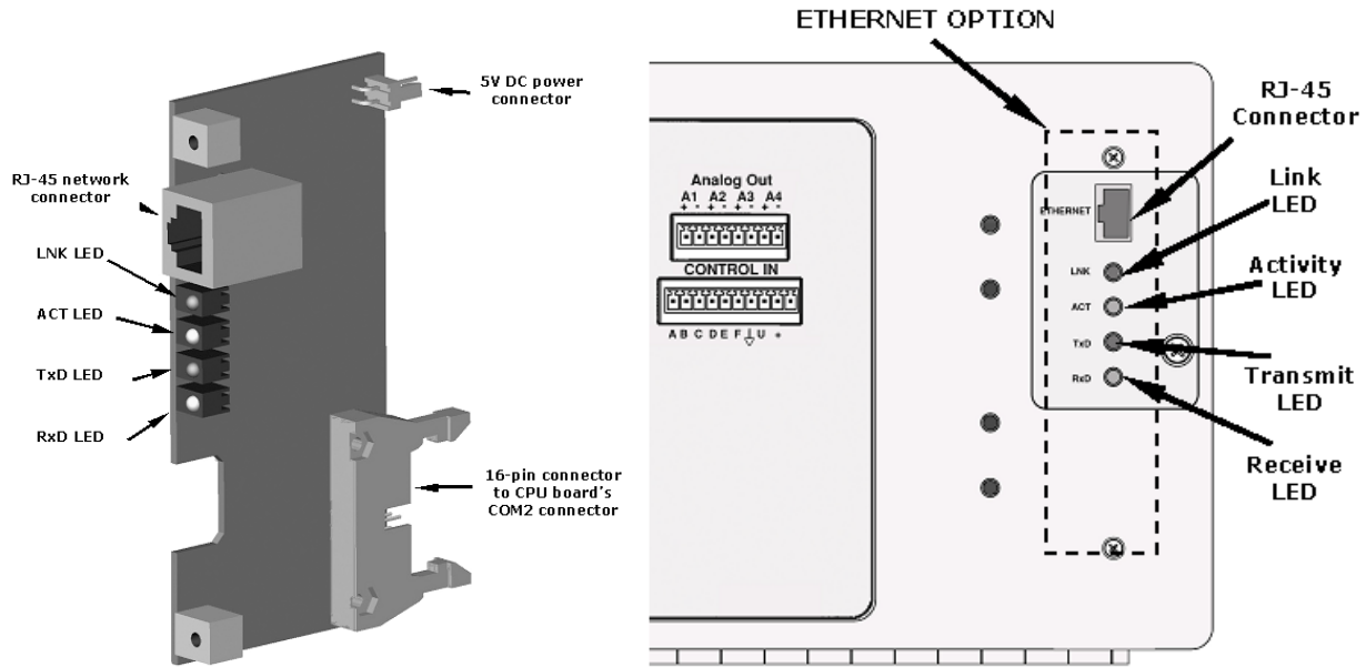
Figure 5-3: M9110EH Ethernet Card and Rear Panel With Ethernet Installed
