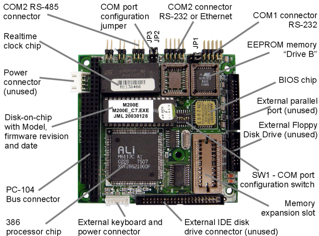
Figure 10-13: Model 9110EH CPU Board Annotated
