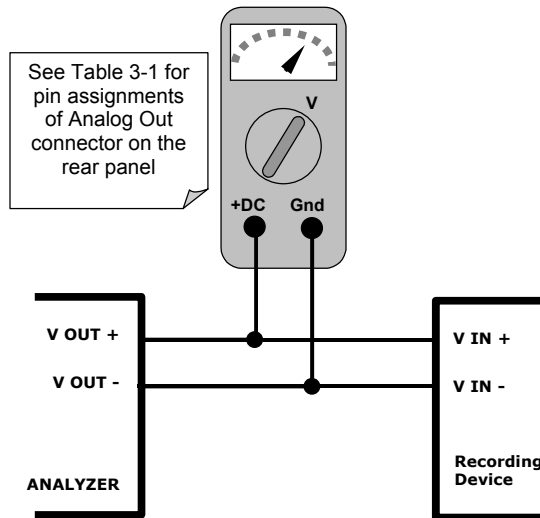
Figure 0-2: Setup for Calibrating Analog Outputs
