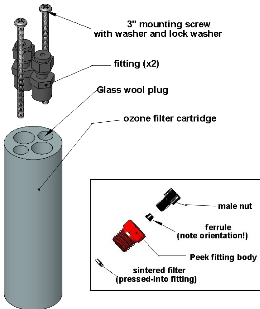
Figure 9-3: Ozone Filter Unit
