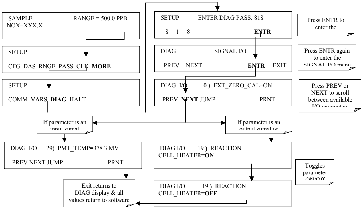
Figure 11-2: Switching Signal I/O Functions
