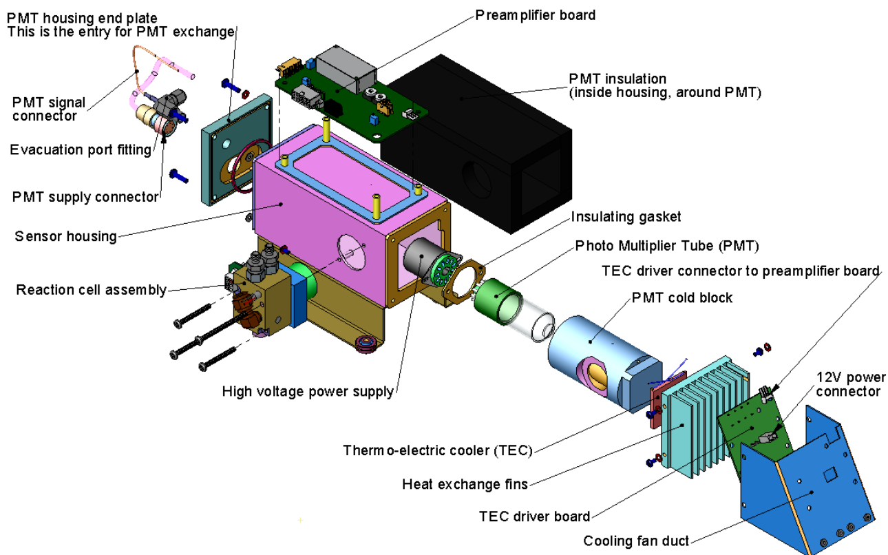
Figure 11-7: Model 9110EH Sensor Assembly
