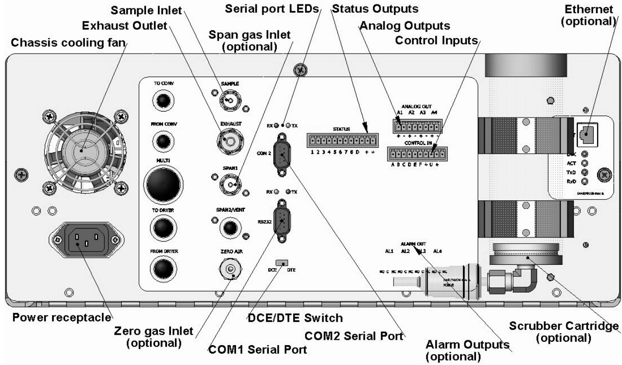
Figure 3-3: M9110EH Rear Panel Layout
