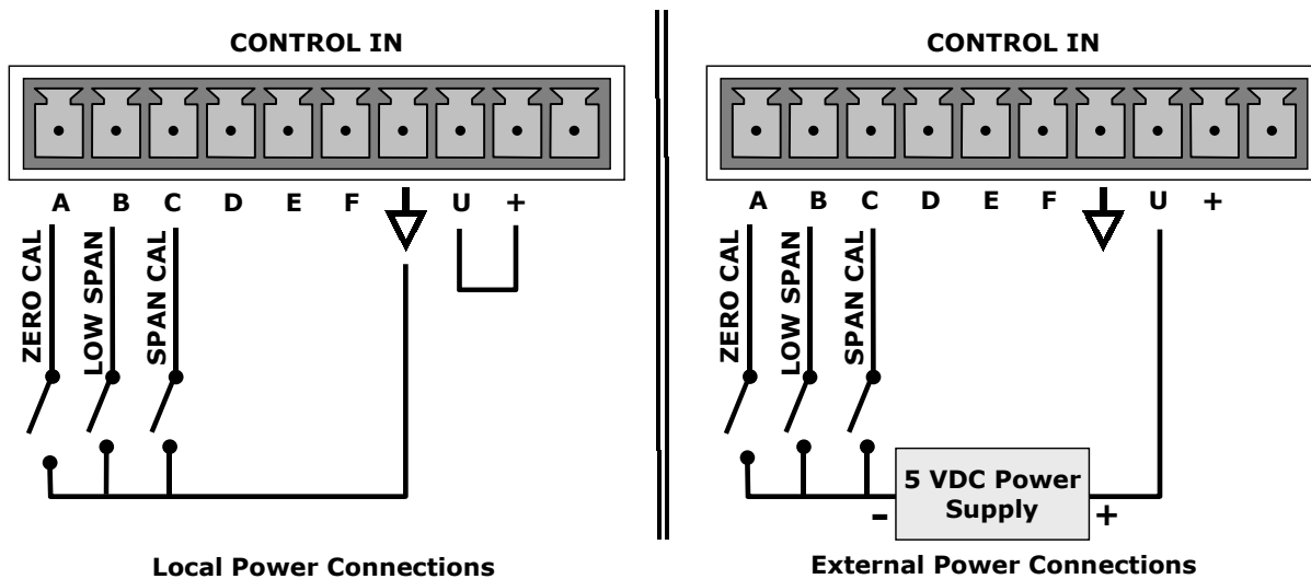
Figure 0-5: Control Inputs with Local and External 5 V Power Supply
