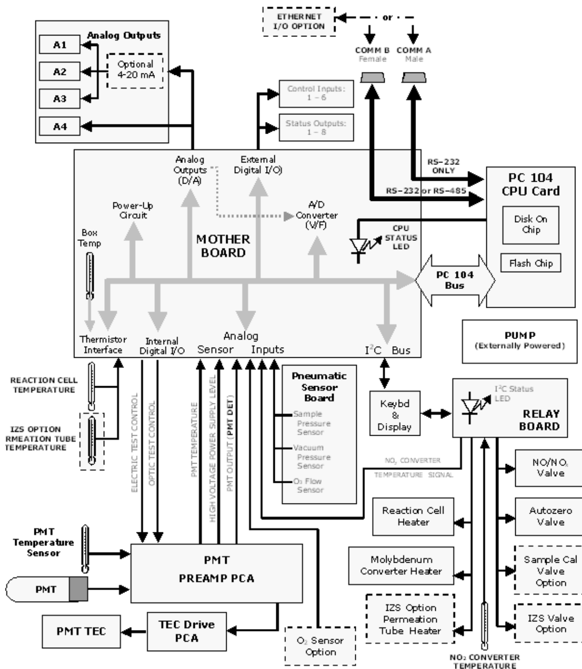
Figure 10-12: Model 9110EH Electronic Block Diagram
