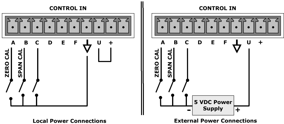
Figure 3-9: Control Input Connector
