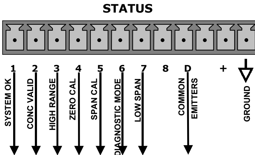
Figure 0-4: Status Output Connector
