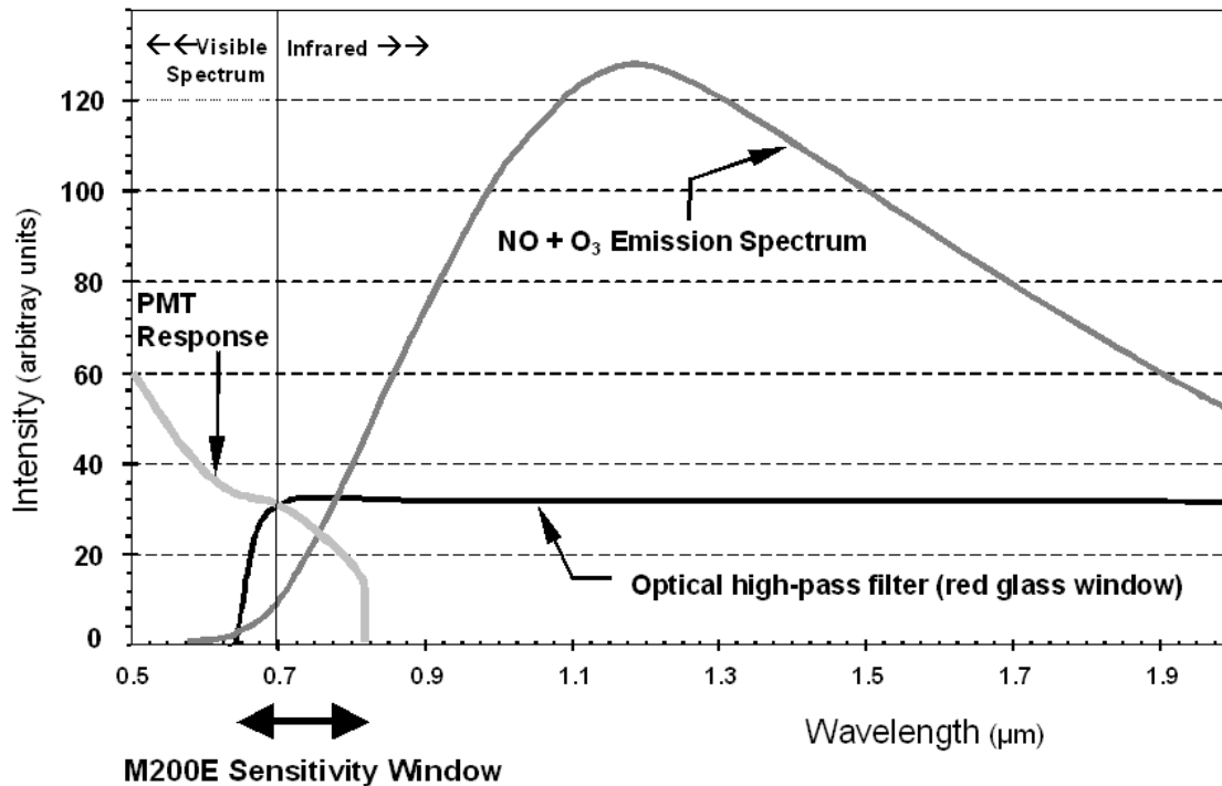
Figure 10-1: M9110EH Sensitivity Spectrum
