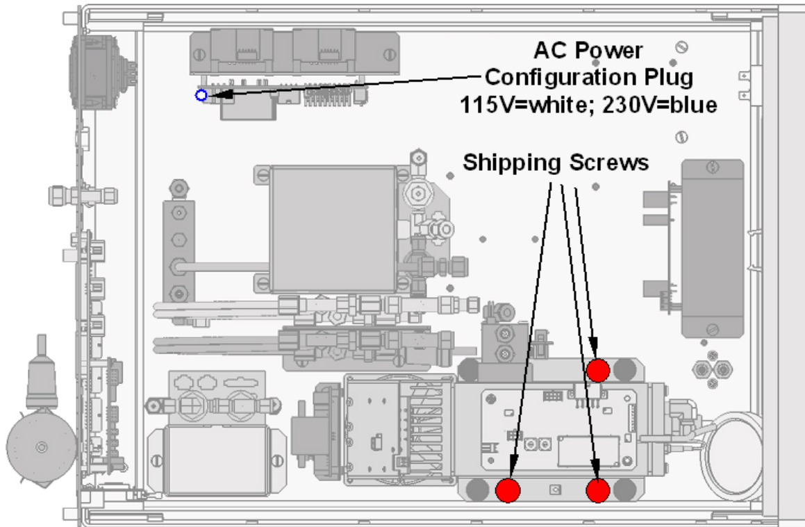
Figure 3-1: Location of Shipping Screws and Power Configuration Plug
