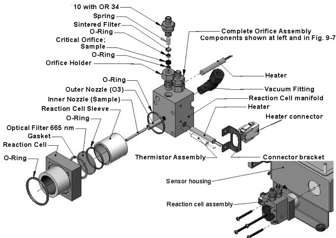
Figure 9-6: Reaction Cell Assembly
