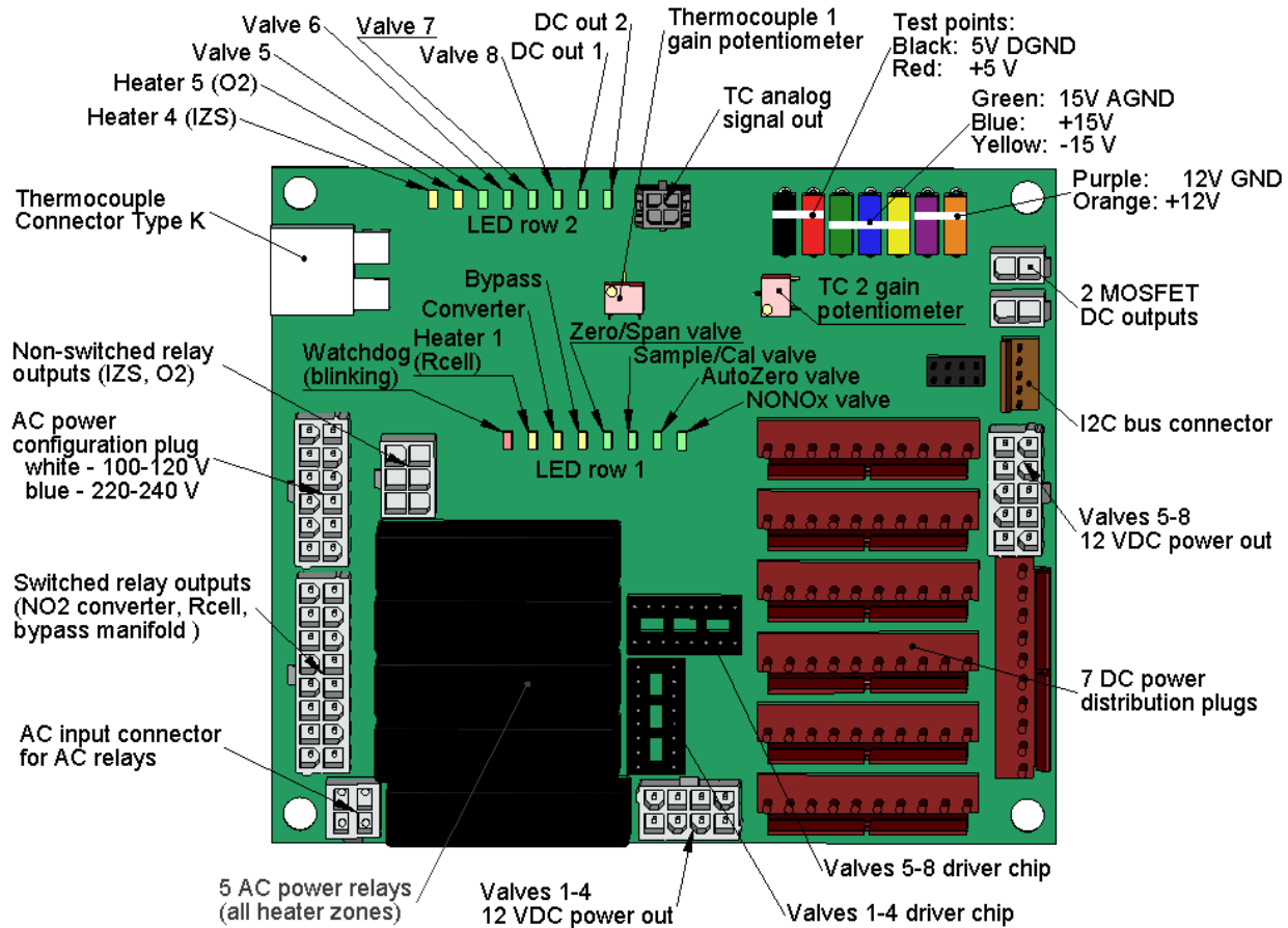
Figure 11-4: Relay Board PCA
