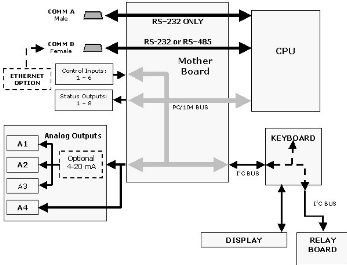
Figure 10-17: Model 9110EH Electronic Interface Block Diagram
