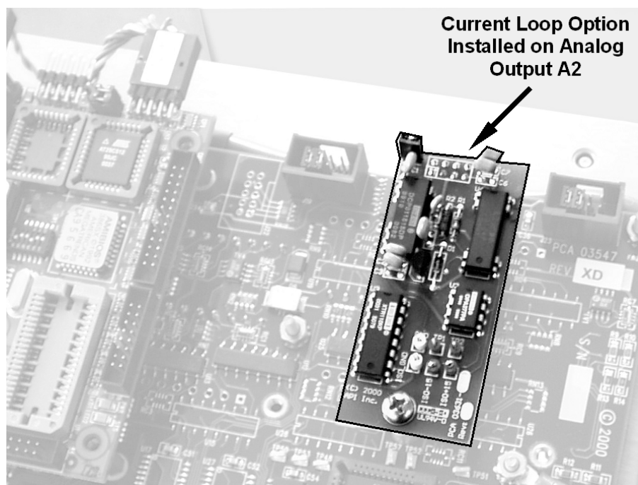
Figure 5-2: Current Loop Option Installed on the Motherboard
