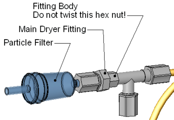
Figure 9-2: Particle Filter on O 3 Supply Air Dryer
