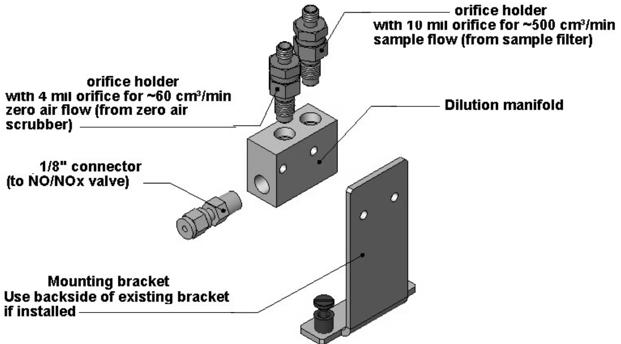
Figure 10-11: Dilution Manifold
