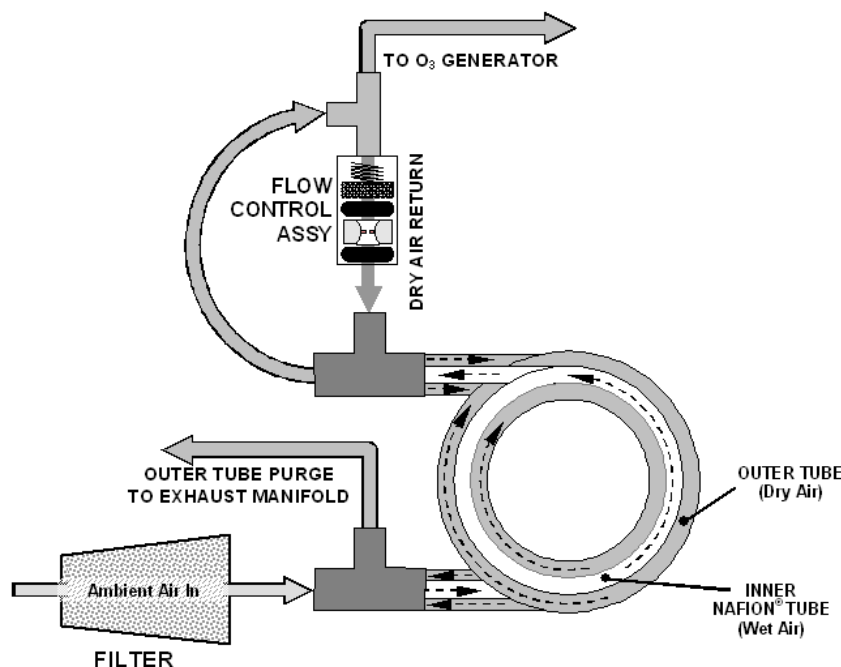
Figure 10-8: M9110EH Perma Pure® Dryer
