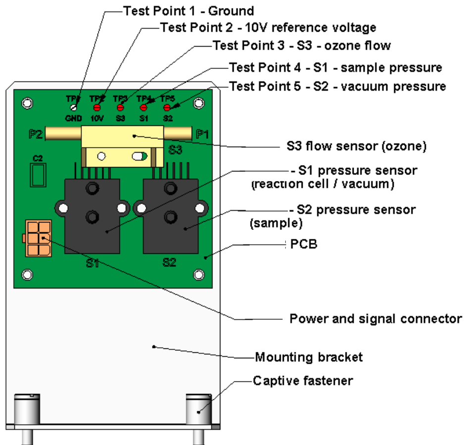
Figure 11-5: Pressure / Flow Sensor Assembly
