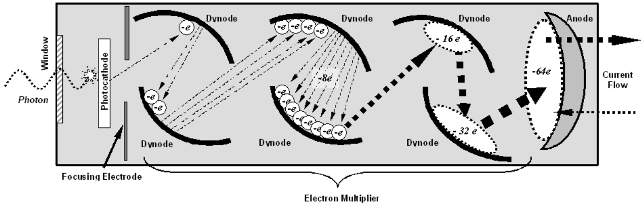
Figure 10-14: Schematic of Basic PMT Design and Functionality
