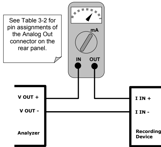
Figure 0-3: Setup for Calibrating Current Outputs
