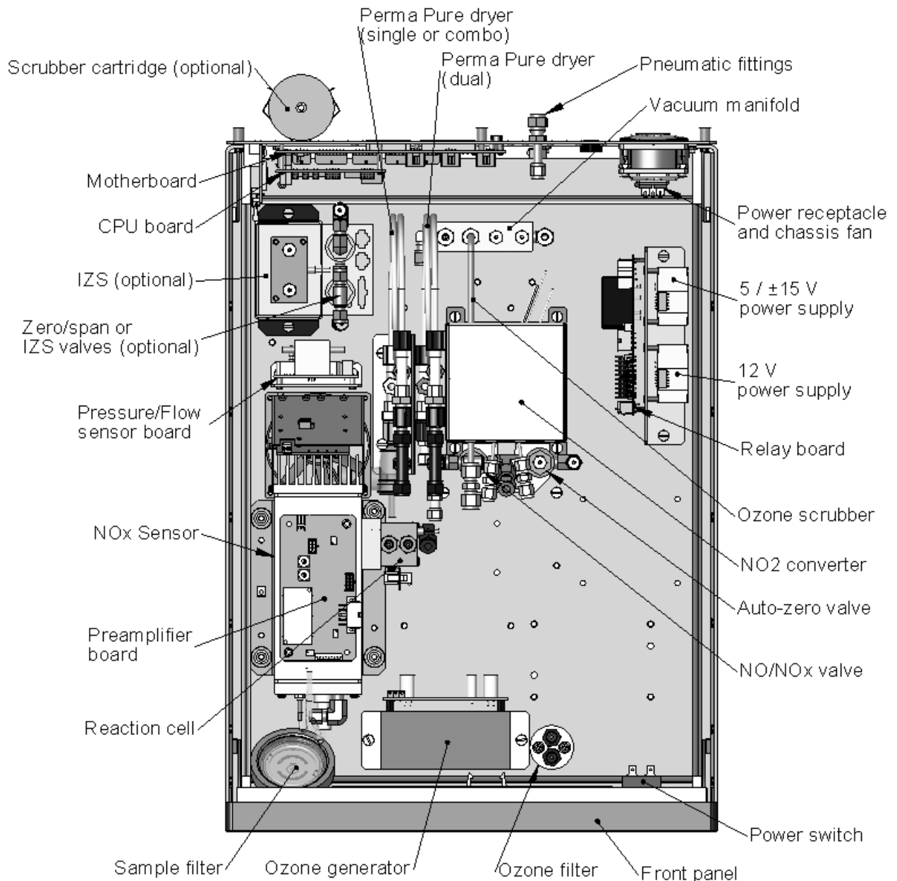
Figure 3-2: M9110EH Layout
